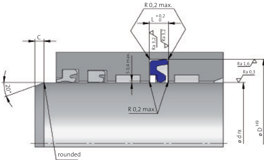
Installation space according to ISO 7425/2 or 5597-1
