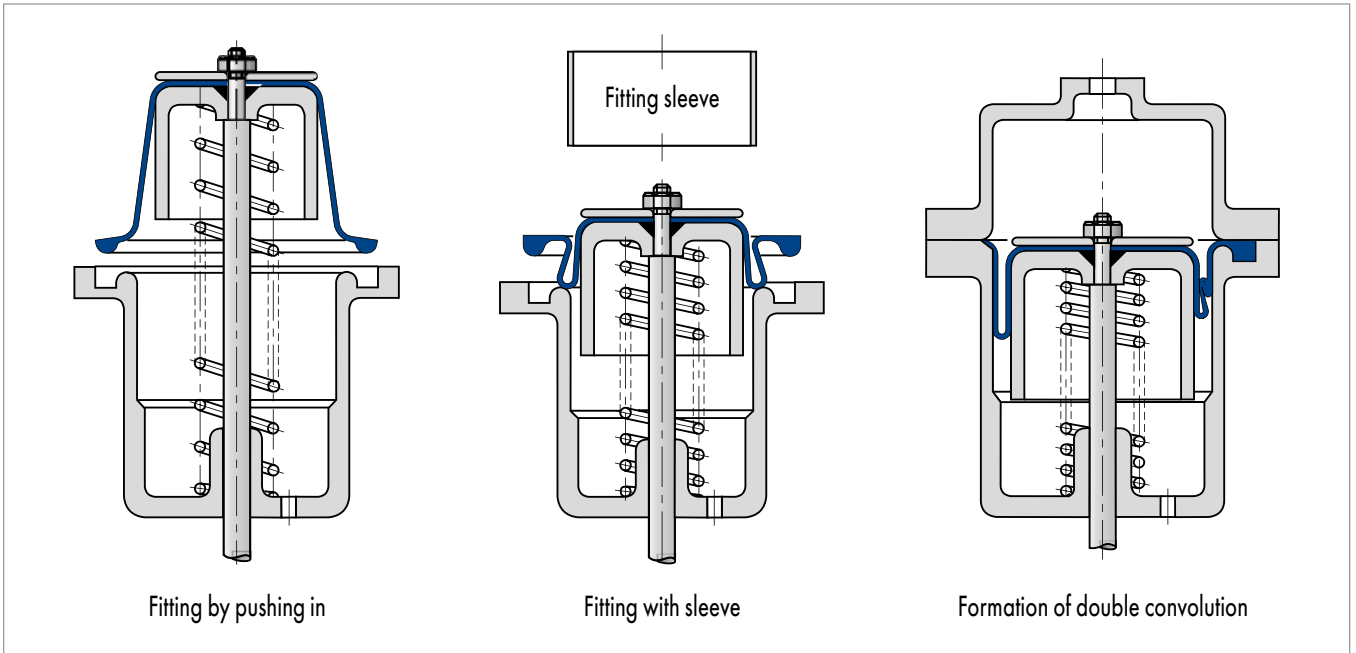
Fitting
